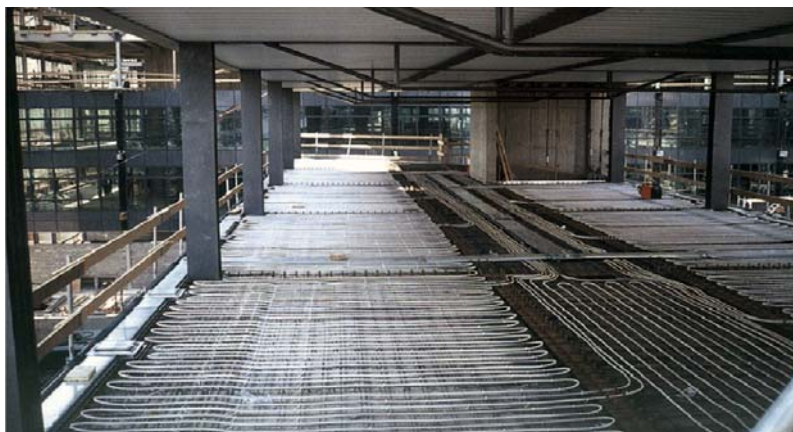
Figure 8: Water heating/cooling pipework placed within the floor slab
